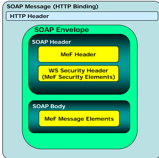
Figure 2-21: Basic SOAP Message Structure for HTTP Binding
